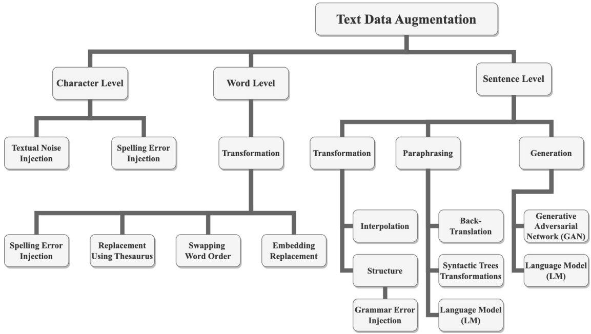
Fig. 1. Taxonomy of Text Data Augmentation Techniques
