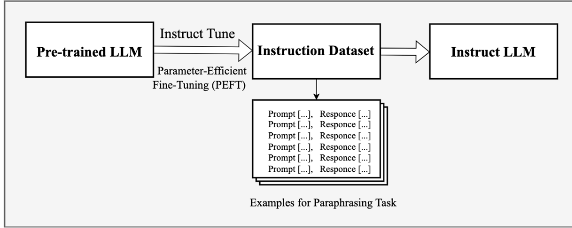
Fig. 4. Instruction fine-tuning of pre-trained Large Language Models (LLMs) for paraphrasing
