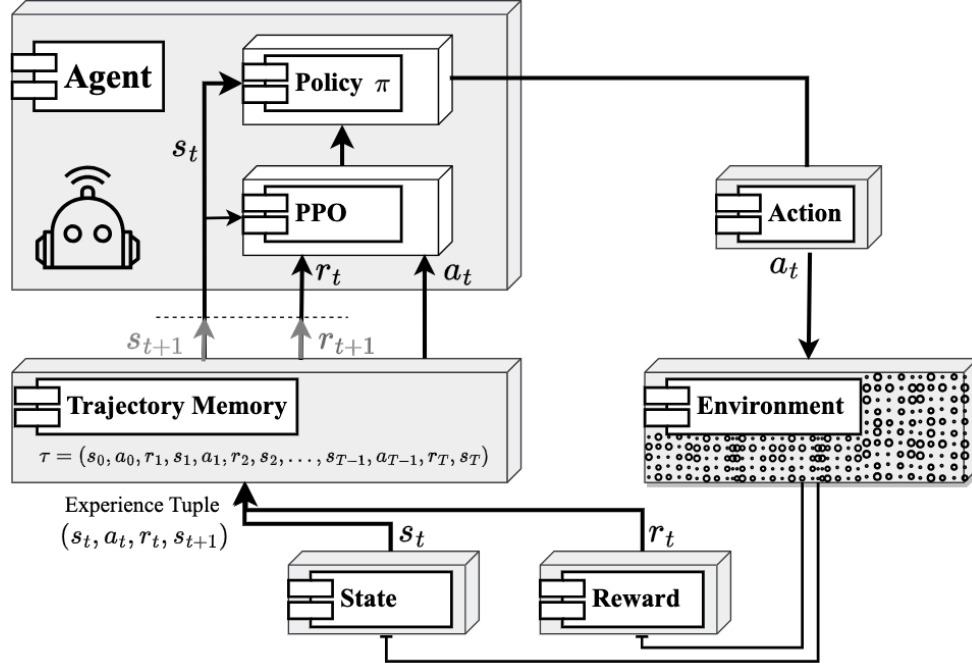
Fig. 2. PPO Model Architecture Overview
